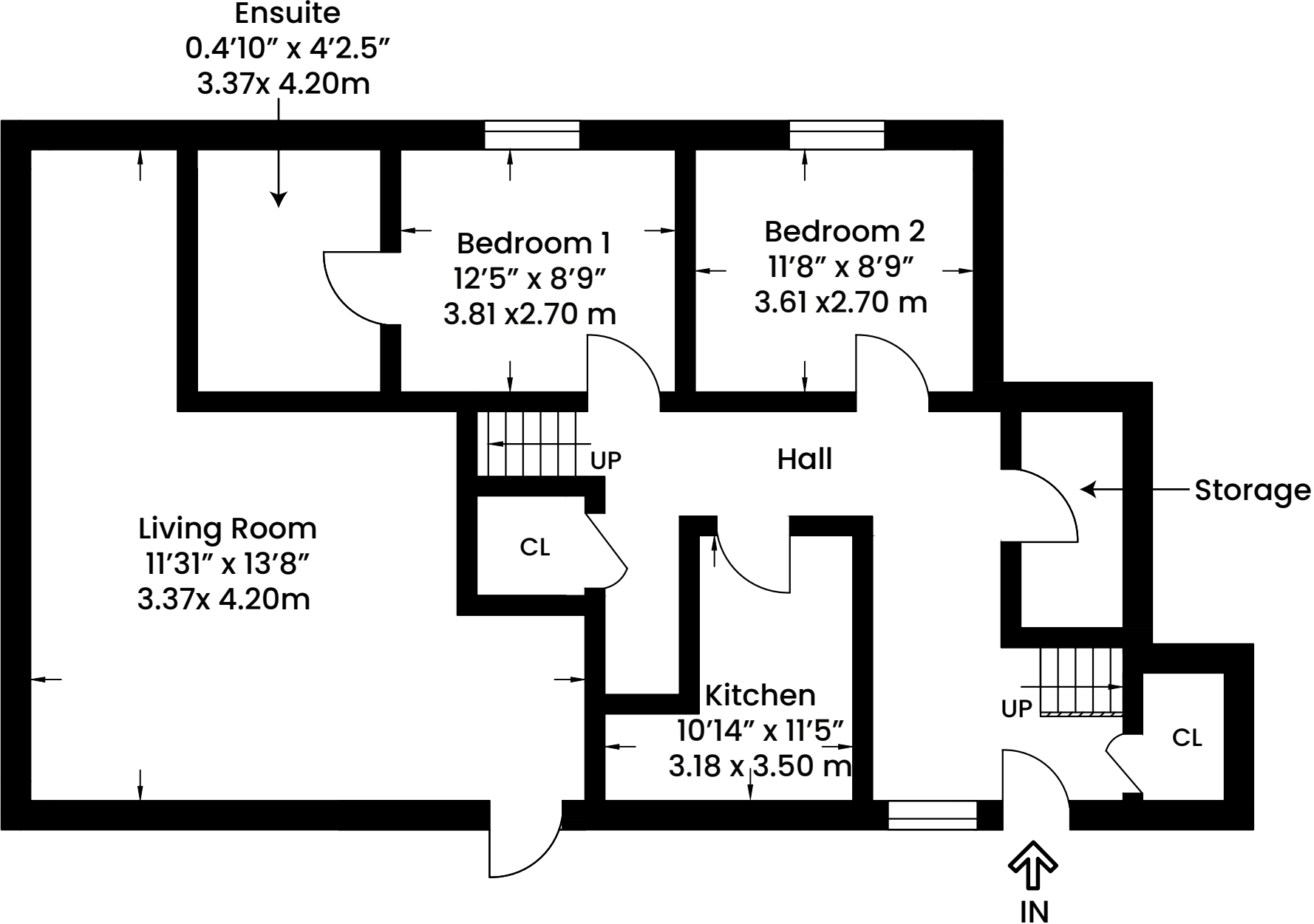
Ground Floor
